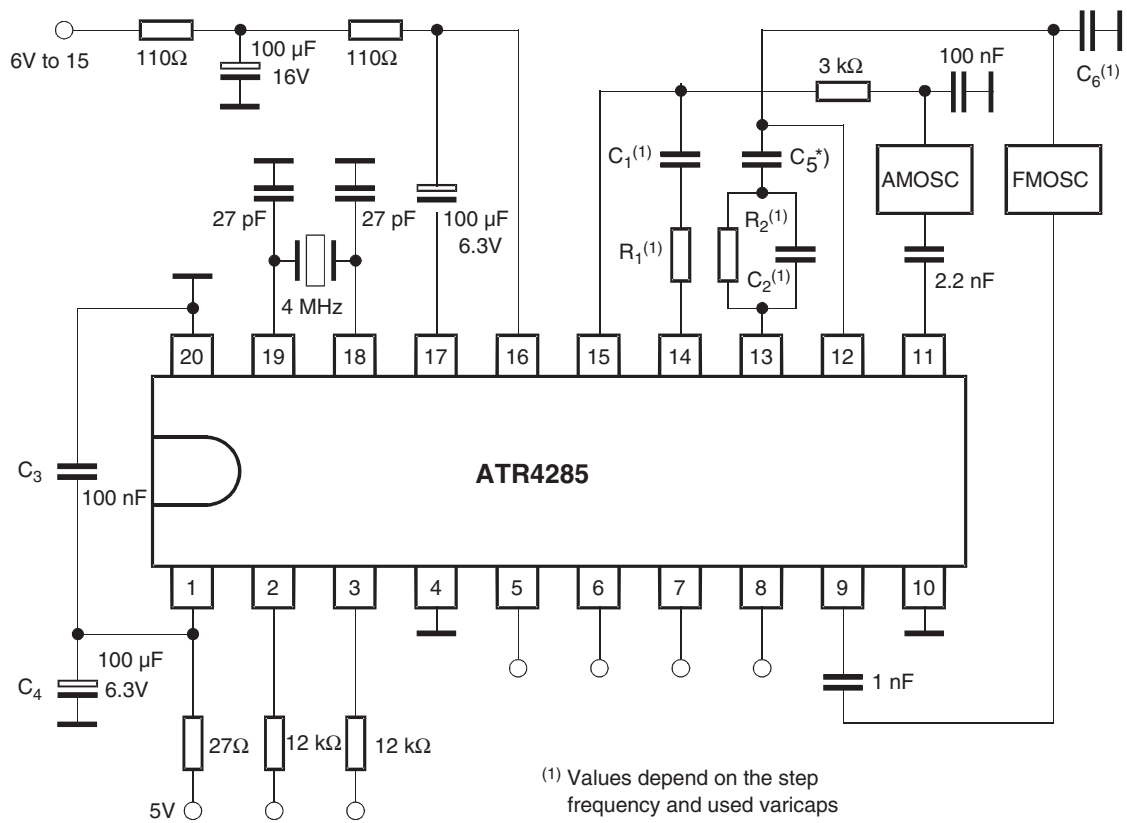
Figure 9-1. Application Circuit
