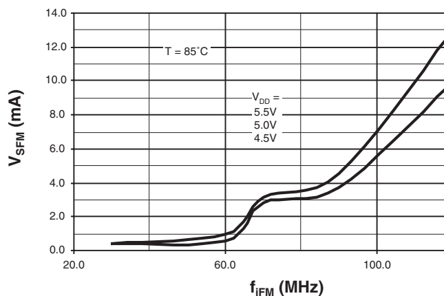
Figure 6-1. FM Input Sensitivity, T = 85^{\circ}\text{C}
