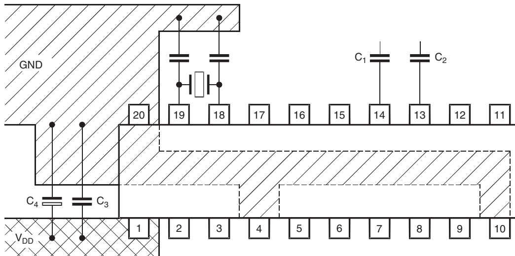
Figure 9-2. PCB Layout
