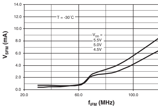
Figure 6-2. FM Input Sensitivity, T = -30^{\circ}\text{C}
